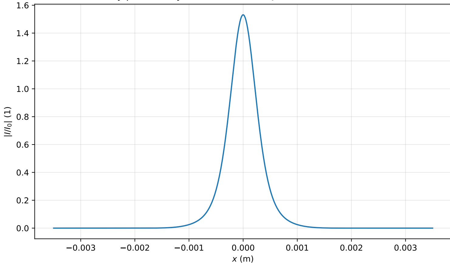
Intensity profile I(x, y = 0, z = 1.353m)/I_0 , P_{in}=0.9P_{cr} , artificial time
